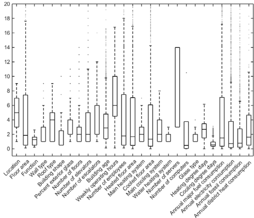
Figure 3: Output of Stage A, distribution of all values of the 27 addressed parameters for 3692 observations.
