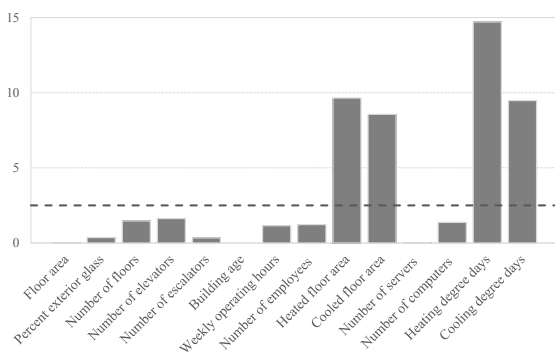
Figure 17: Variance inflation factors for the predictor parameters of the subset of buildings categorized by building age. The category used as an example is buildings built after 1999.
