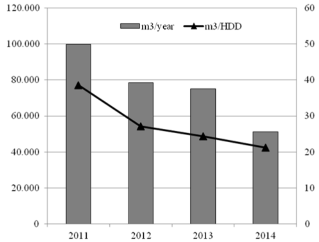
Figure 4: Annual gas consumption for the Strukton office building in Son in total and normalized by degree days. Because only one building was looked at, and its floor area did not change in time, normalization by floor area was not carried out.
